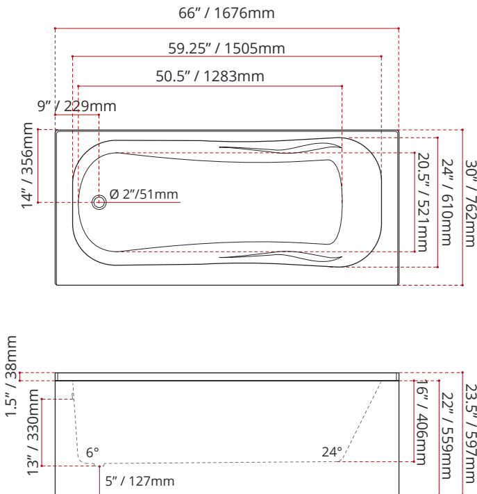
MODEL NUMBER : 4331 (LEFT HAND DRAIN LOCATION)
