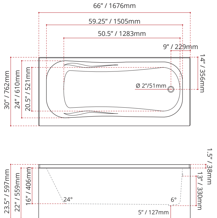
MODEL NUMBER : 4341 (RIGHT HAND DRAIN LOCATION)
